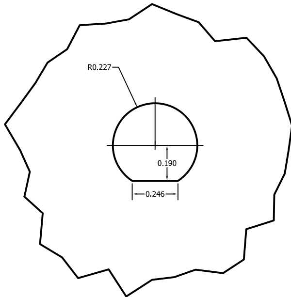
DETAIL A SCALE 4
