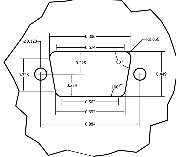
DETAIL B SCALE 4
